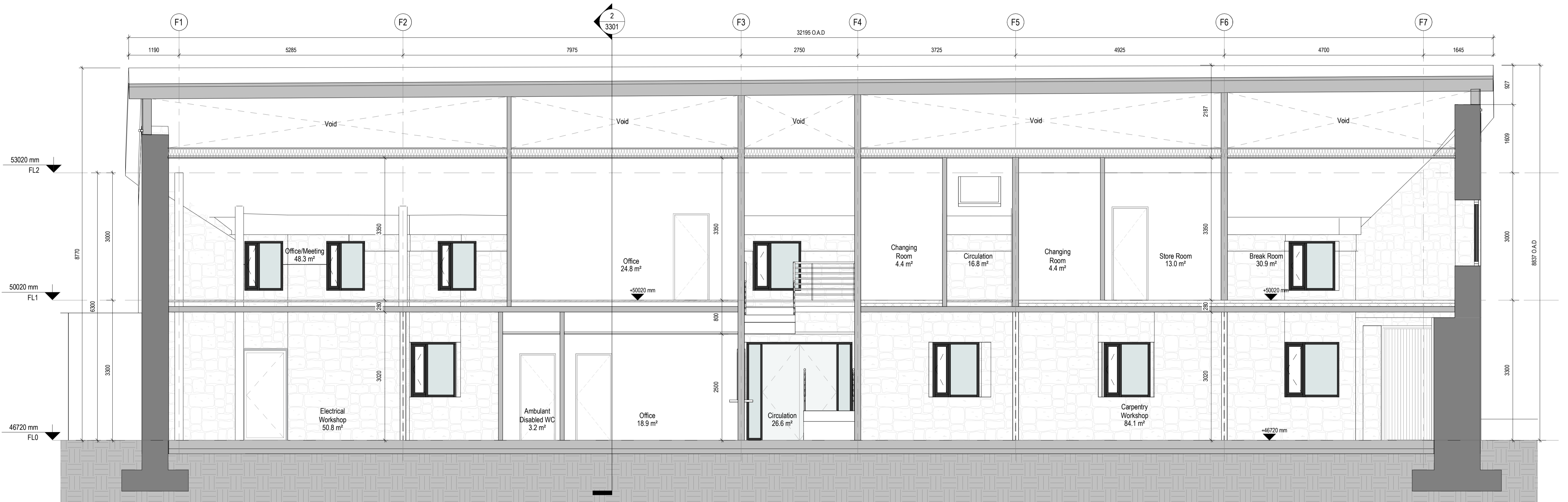
1 Section North South 3301 Scale: 1 : 50
