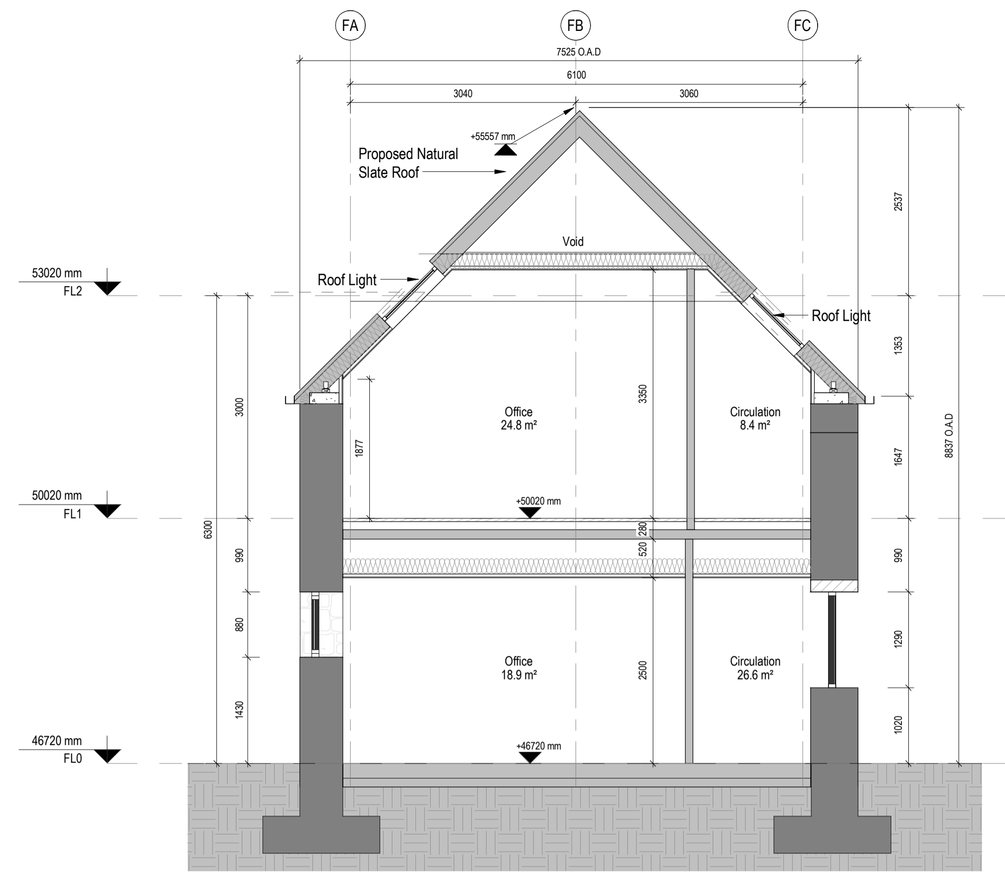
2 Section East West 3301 Scale: 1 : 50
